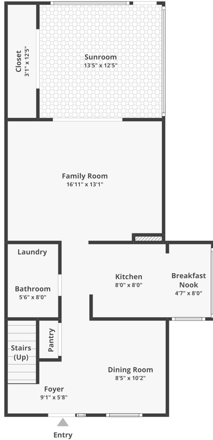
FLOOR 1
